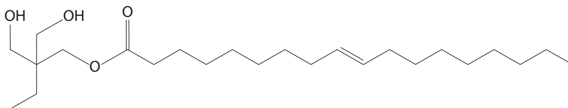
compound X
