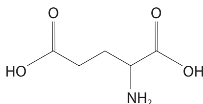
glutamic acid
