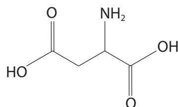
aspartic acid
